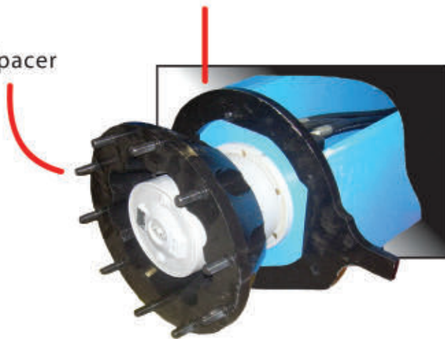
Anti-rotation Bracket
